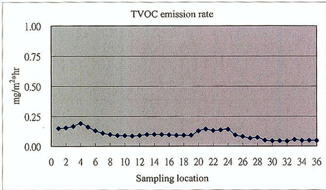
Fig1. TVOC emission rate of building materials
